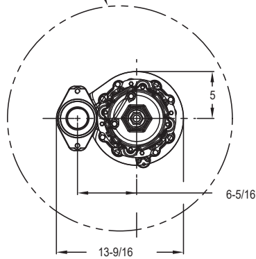
SIMPLEX INSTALLATION
